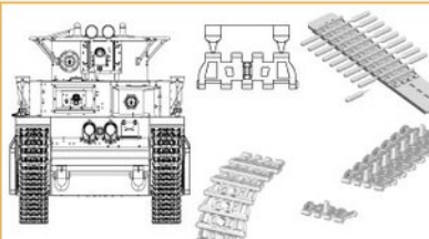
Soviet T-35 Heavy Tank Track Links 苏联T-35重型坦克活动履带
